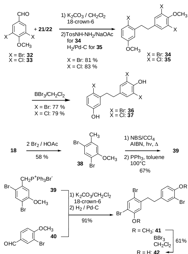
Scheme 6 Syntheses of trihalogenated lunularins
